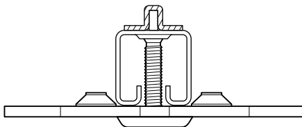
Installed Profile
