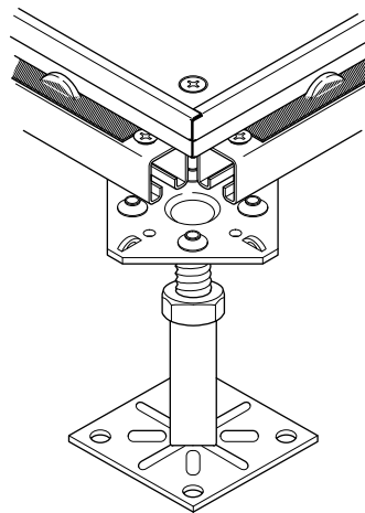
Corner-Lock Application
